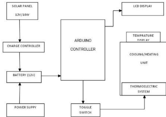
Fig 4.1. Solar Powered Thermo-Electric Refrigeration cum Oven System
