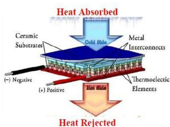
Figure 5.1: Operating principle of thermo- electric module (adapted from scientific and production firm module -ISO 9001)
